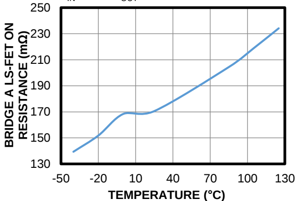
Bridge A LS-FET On Resistance vs. Temperature
