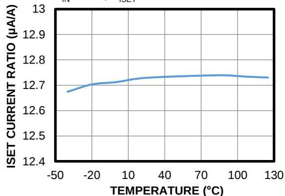
ISet Current Ratio vs. Temperature
