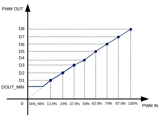
Figure 5: Curve Configuration
