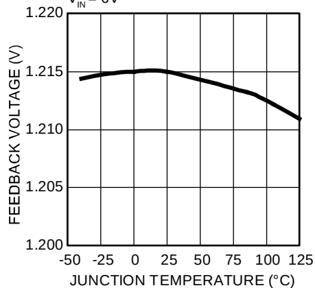
Feedback Voltage vs. Junction Temperature
