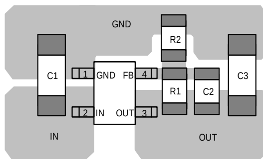
Figure 10: Recommended PCB Layout (Top Layer)
