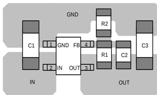
Figure 10: Recommended PCB Layout (Top Layer)
