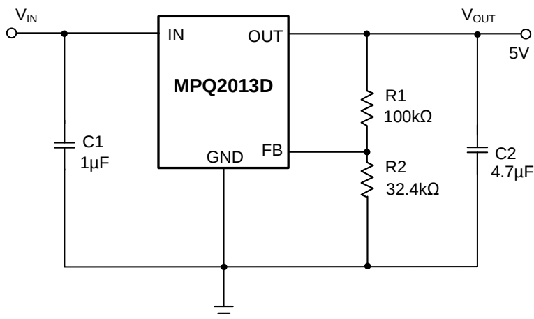
Figure 13: Typical Application Circuit (5V Output)
