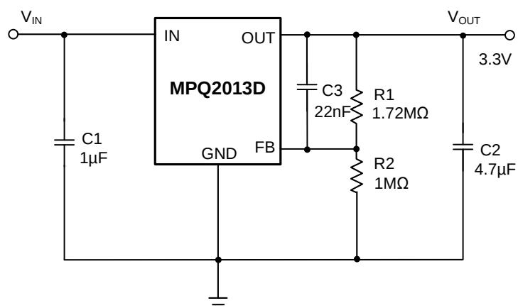
Figure 11: Typical Application Circuit (3.3V Output with Feed-Forward Capacitor)
