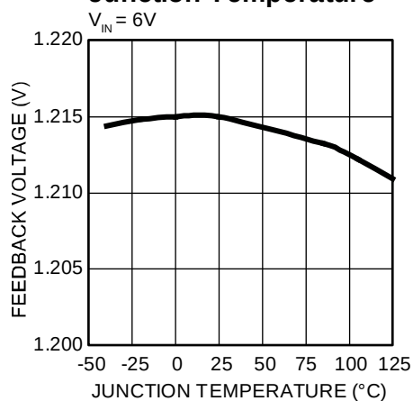
Feedback Voltage vs. Junction Temperature V_{IN} = 6V
