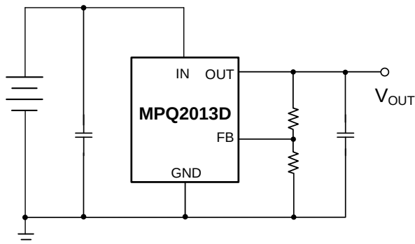
Figure 1: Adjustable-Output Version
