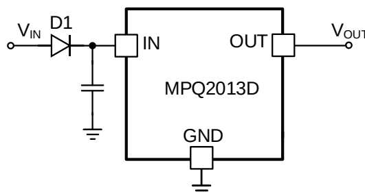
Figure 7: External Reverse-Voltage Protection
