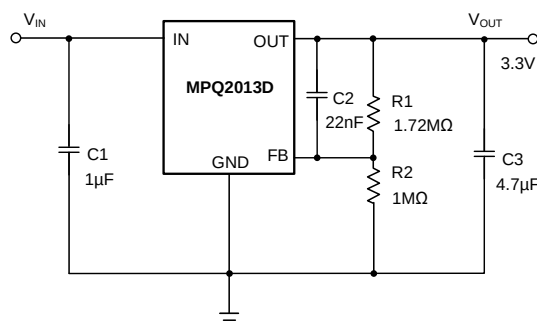
Figure 8: Design Example
