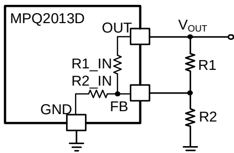
Figure 6: FB Divider for Fixed V OUT Version
