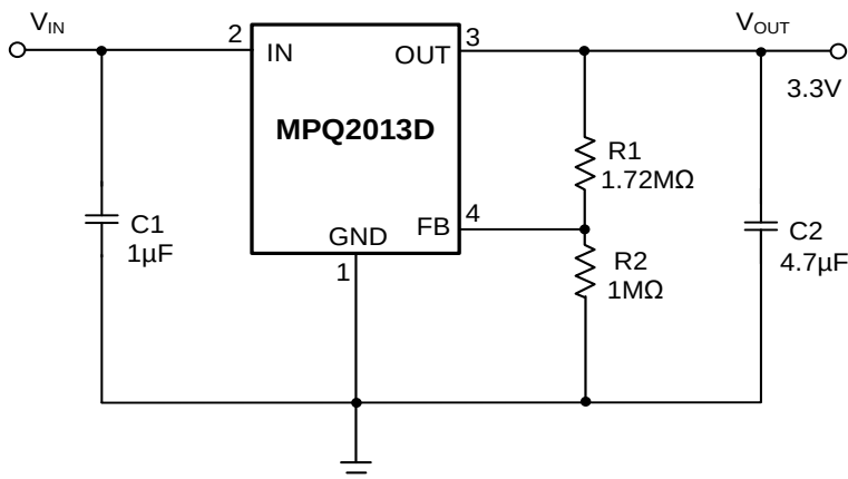
Figure 4: Typical Application Circuit (V OUT = 3.3V)
