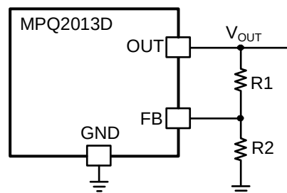
Figure 5: FB Resistor Divider Sets V OUT
