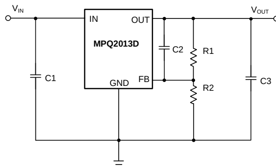
Figure 9: Typical Application Circuit
