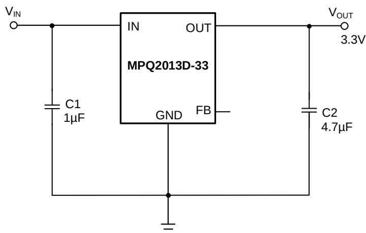
Figure 12: Typical Application Circuit (3.3V Fixed Output)
