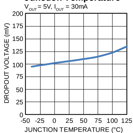
Dropout Voltage vs. Junction Temperature V_{OUT} = 5V , I_{OUT} = 30mA
