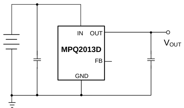
Figure 2: Fixed-Output Version
