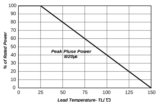
Fig3.Power Derating Curve
