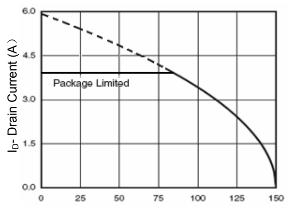
Figure 4 Drain Current
