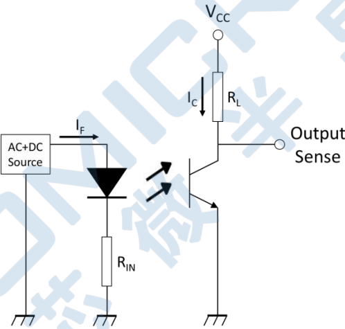
Fig.14 Test Circuits of Frequency Response
