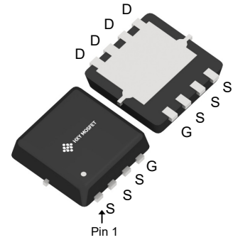
DFN3X3-8L (PowerFLAT-8(3.3x3.3))
