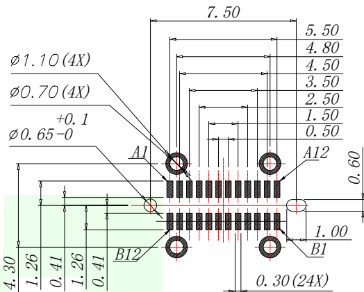
RECOMMENDED PCB LAYOUT (TOP VIEW) THICKNESS 1.0±0.10MM; DEFAULT TOLERANCE: ±0.05
