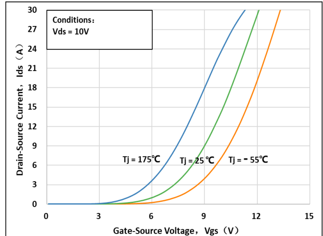
Fig 6: Transfer Characteristic
