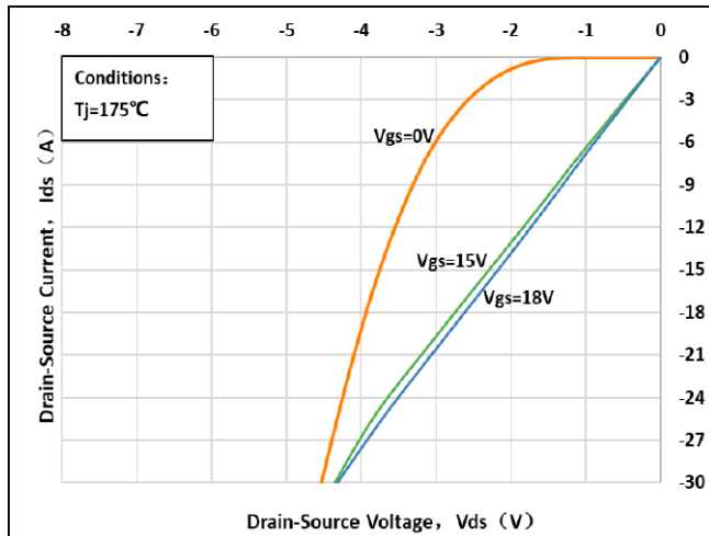
Fig 13: 3rd Quadrant Characteristic( T_J=175^{\circ}\text{C} )
