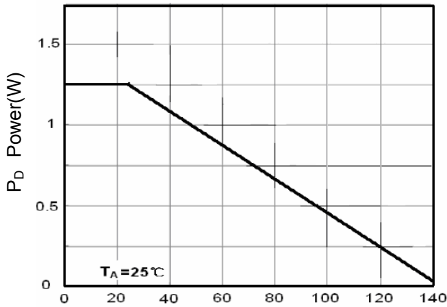
T_J -Junction Temperature( ^{\circ}C ) Figure 3 Power Dissipation
