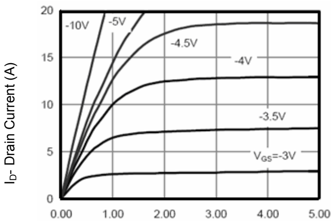
V_{DS} Drain-Source Voltage (V) Figure 5 Output Characteristics
