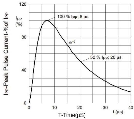
IEC61000-4-5 8X20 \mu\text{s} Pulse Waveform
