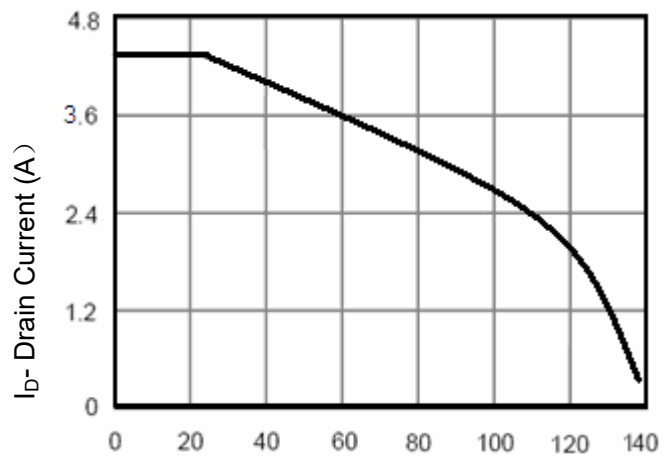
T_J -Junction Temperature( ^{\circ}C ) Figure 2 Drain Current
