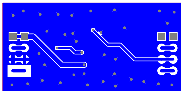
Figure 32. ZJR1001 Evaluation Board Layout (Bottom Layer)
