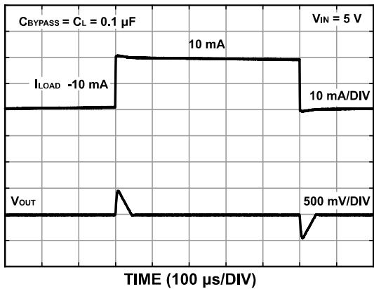
Figure 22. ZJR1002-9 Load Transient
