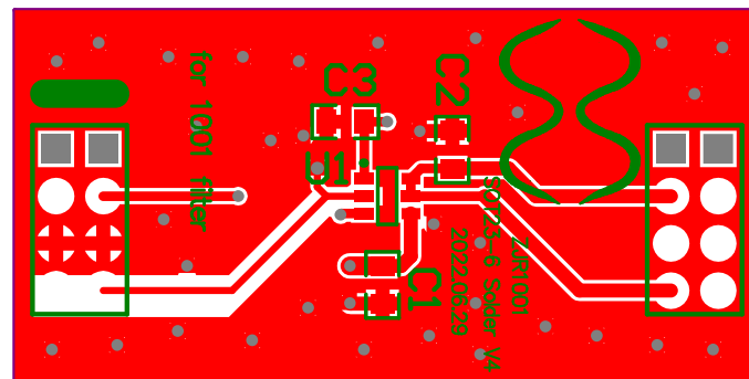
Figure 31. ZJR1001 Evaluation Board Layout (Top Layer)
