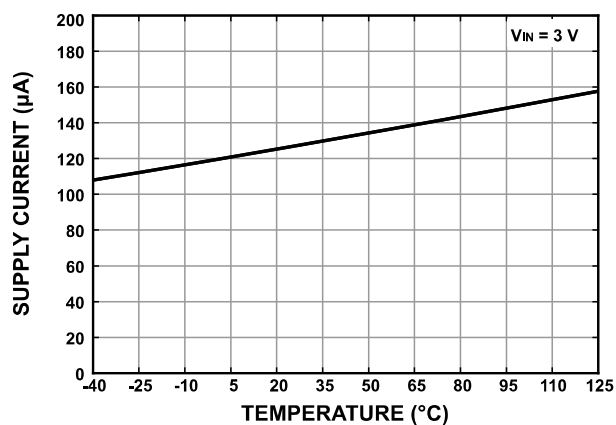
Figure 12. ZJR1002-9 Supply Current vs. Temperature
