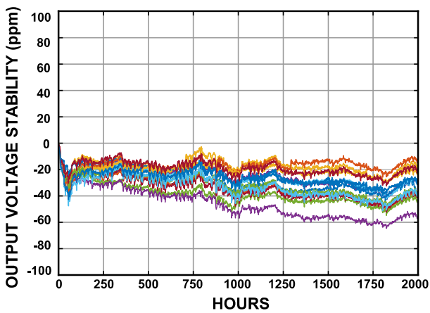
Figure 25. Long-Term Stability
