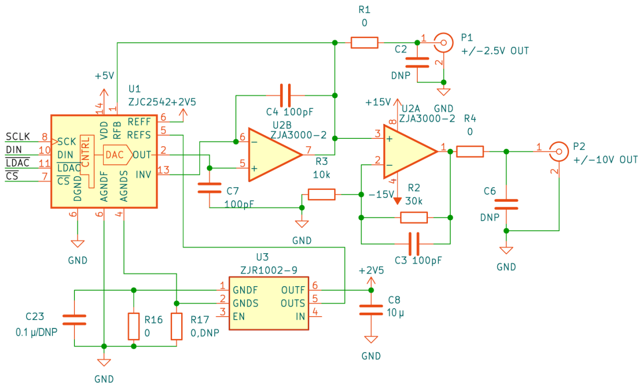
Figure 29. ZJR1002 and ZJC2542 build 18-bit programmable signal source
