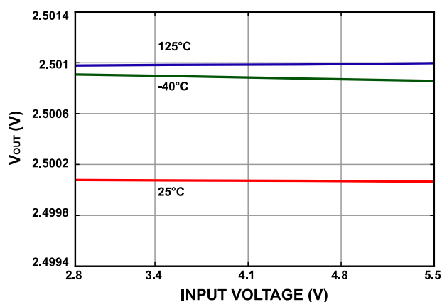
Figure 13. ZJR1002-9 Line Regulation
