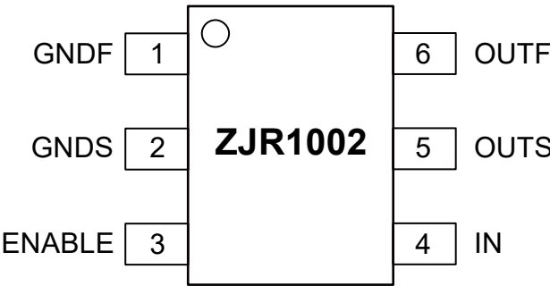
Figure 2. ZJR1002 Pin Configuration (6-lead SOT23)
