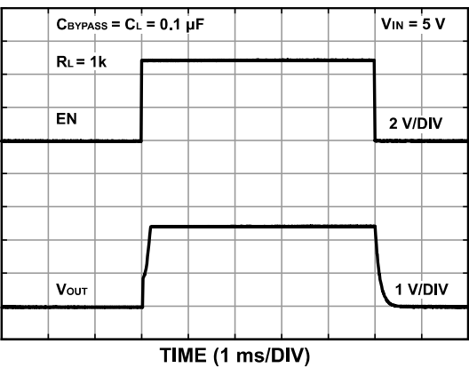
Figure 20. ZJR1002-9 Enable Transient
