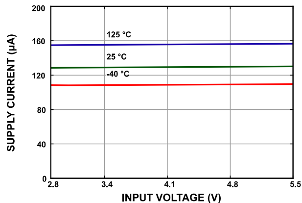
Figure 10. ZJR1002-9 Supply Current vs. Input Voltage
