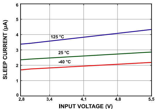
Figure 11. ZJR1002-9 Shutdown Current vs. Input Voltage
