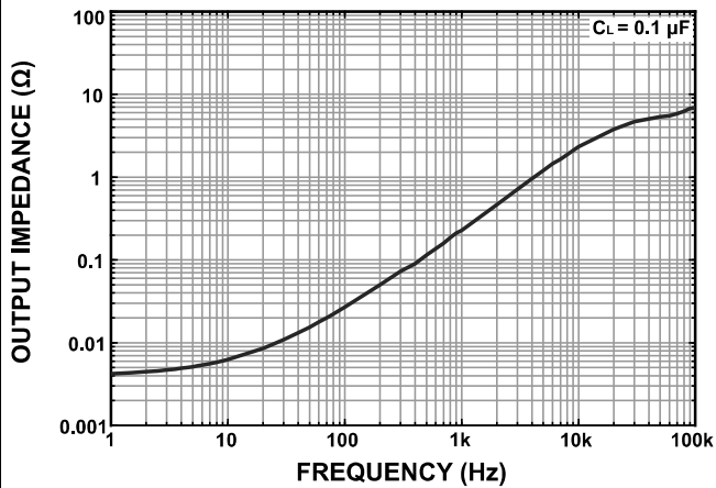
Figure 24. ZJR1002-9 Output Impedance vs. Frequency
