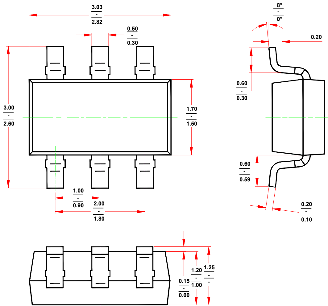
Figure 33. 6-Lead SOT23 Package Dimensions shown in millimeters
