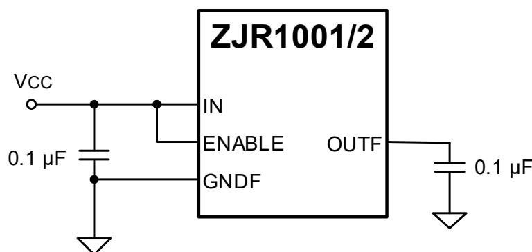
Figure 28. ZJR1001/2 Basic Connections
