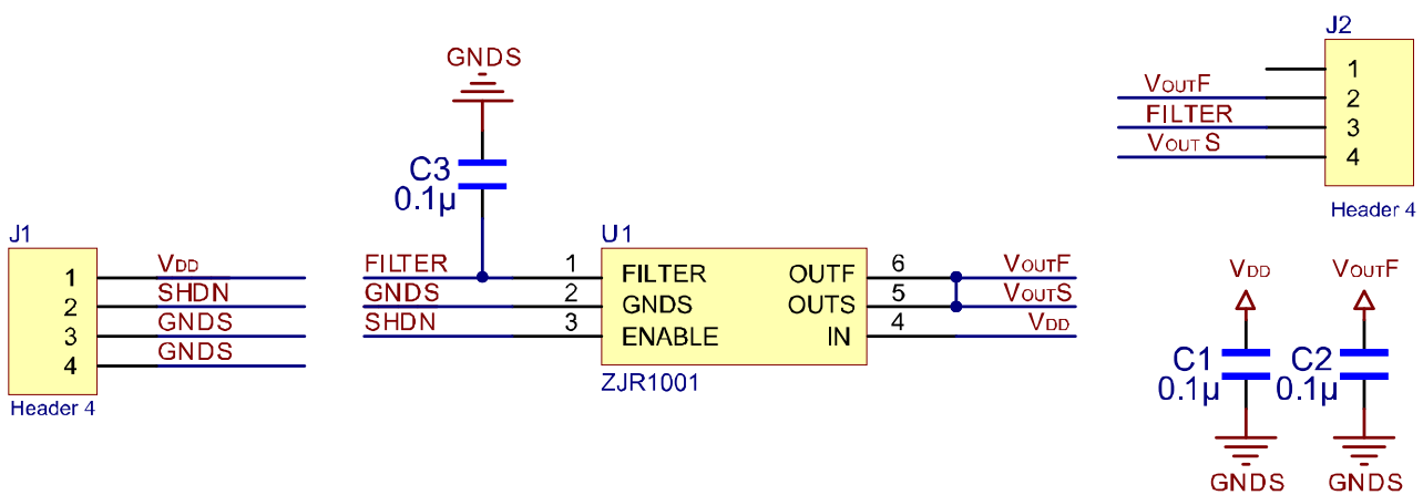
Figure 30. ZJR1001 Evaluation Board Schematic
