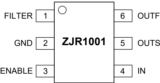
Figure 1. ZJR1001 Pin Configuration (6-lead SOT23)
