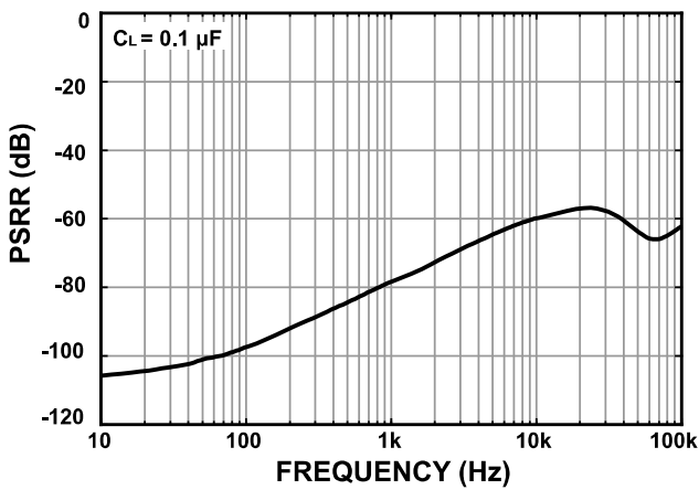
Figure 23. ZJR1002-9 Power Supply Rejection Ratio vs. Frequency
