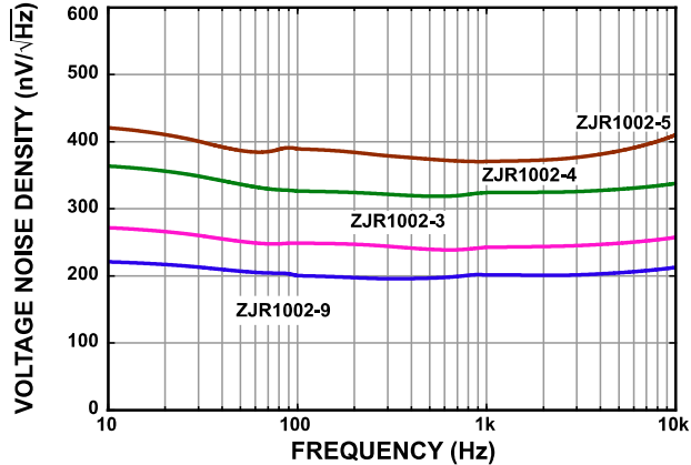
Figure 16. ZJR1002 Noise Density vs. Frequency
