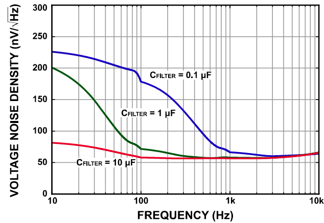
Figure 17. ZJR1001-9 Noise Density vs. Frequency
