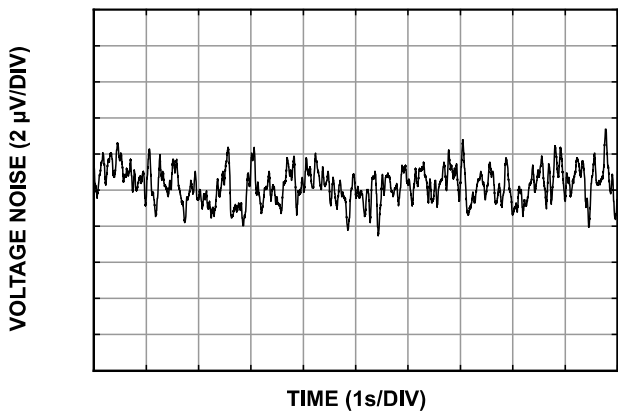
Figure 15. ZJR1002-9 Typical Voltage Noise (0.1 Hz to 10 Hz)
