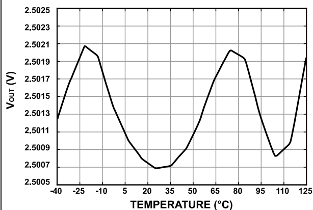
Figure 9. ZJR1002-9 Typical Output Voltage vs. Temperature
