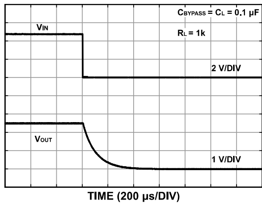
Figure 19. ZJR1002-9 Turn-Off Response
