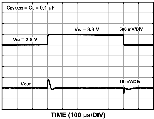
Figure 21. ZJR1002-9 Line Transient
