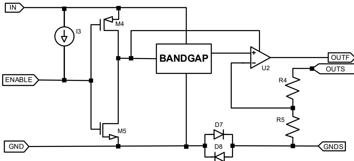
Figure 27. Simplified Schematic of ZJR1002
