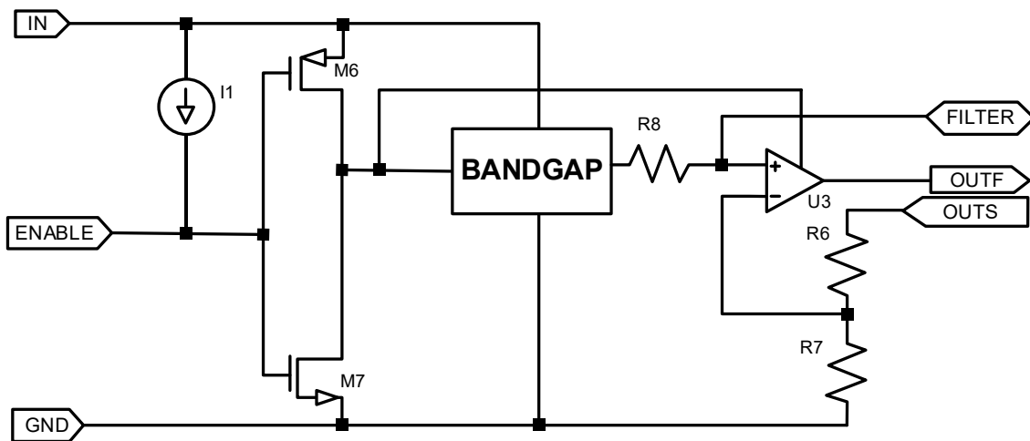
Figure 26. Simplified Schematic of ZJR1001
