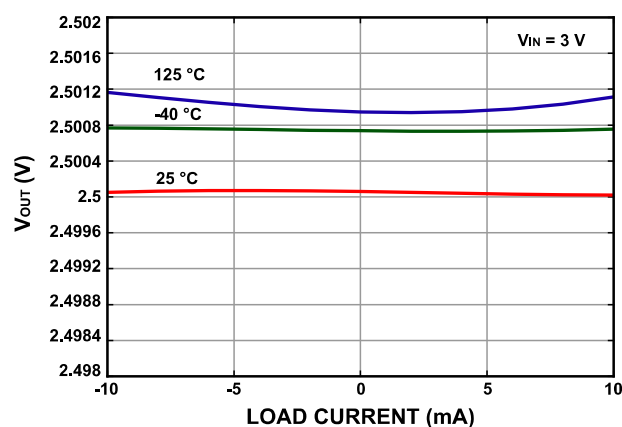
Figure 14. ZJR1002-9 Load Regulation
