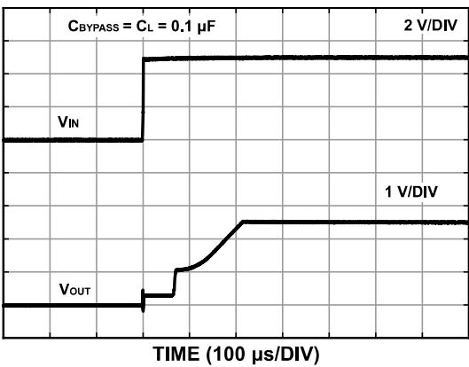
Figure 18. ZJR1002-9 Turn-On Response
