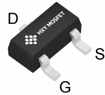
SOT-23-3L (SOT-23F)
