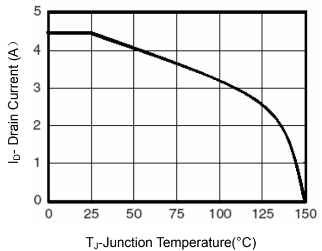
Figure 4 Drain Current
