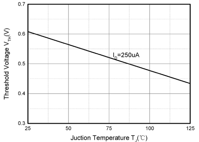
Threshold Voltage
