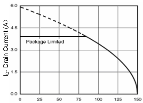
Figure 4 Drain Current
