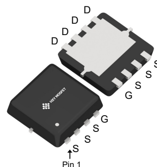
DFN3X3-8L (TSDSON-8(3.3x3.3))
