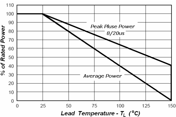
Fig 2.Power Derating
