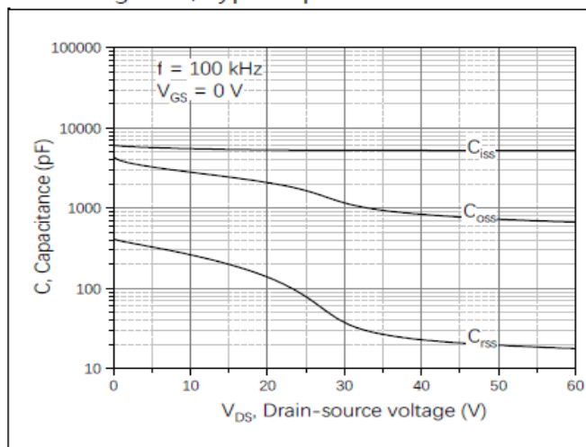
Figure 3, Typ. capacitances
