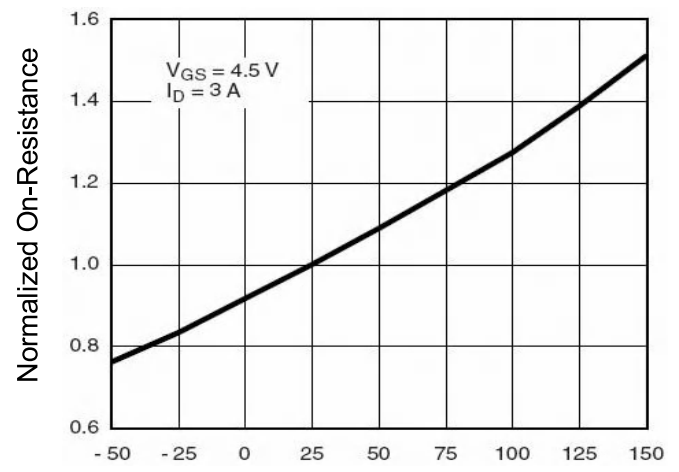
Figure 8 Drain-Source On-Resistance
