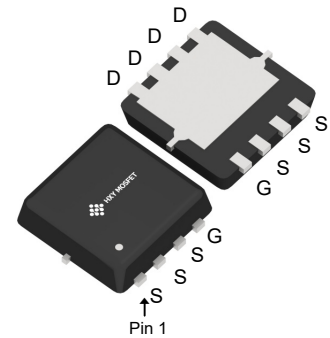
DFN3X3-8L (VSONP-8(3.3x3.3))
