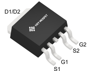
TO-252-4L (TO-252-4)
