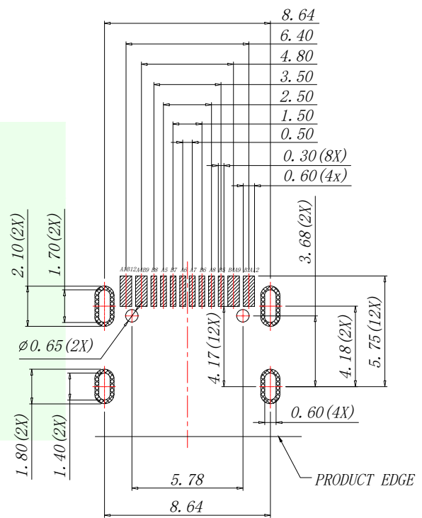
RECOMMENDED PCB LAYOUT (TOP VIEW) THICKNESS 1.00MM; DEFAULT TOLERANCE: ±0.05
