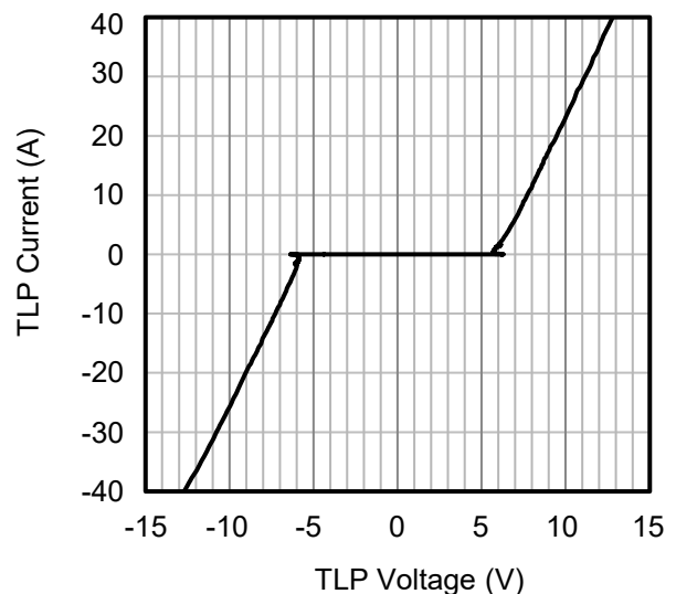
Fig4. TLP Measurement
