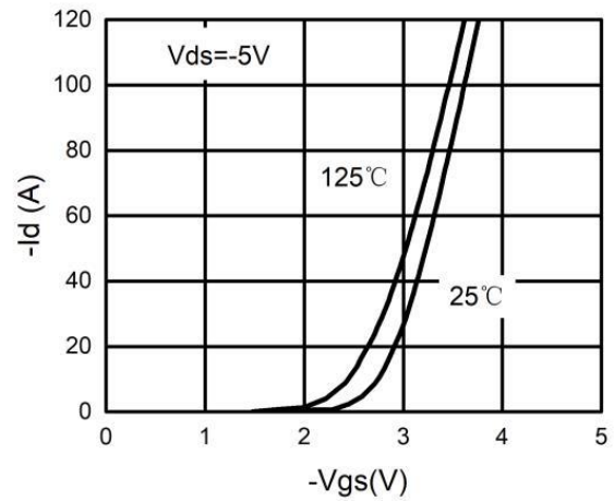
Figure 4. Drain Current
