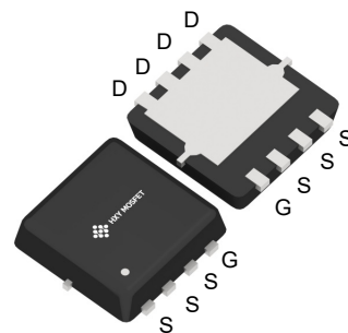
DFN3X3-8L
