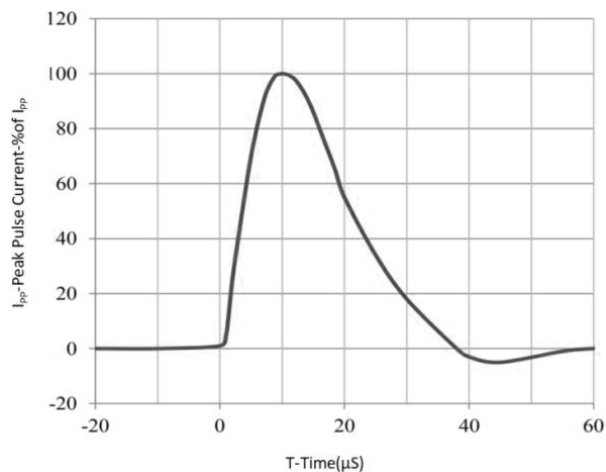
EC61000-4-5 Waveform( 8/20 \mu s pulse)
