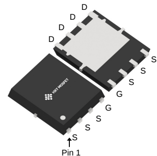
DFN5X6-8L (TDSON-8)
