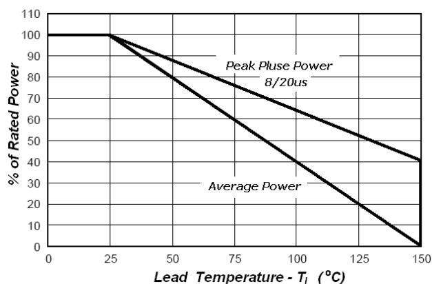
Fig 2. Power Derating
