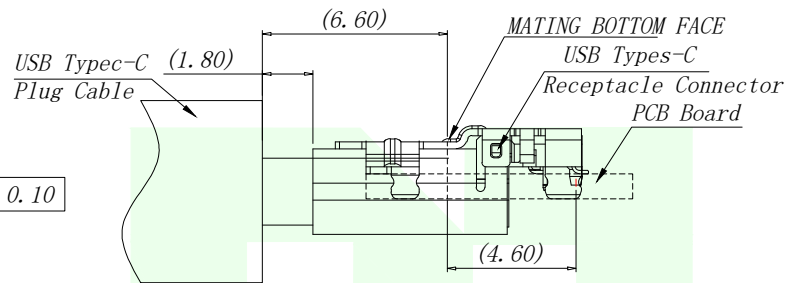
MATED CONDITION SCALE 1:1
