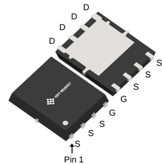
DFN5X6-8L (DFN(5x6))
