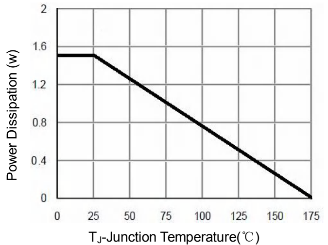
Figure 10 Power De-rating
