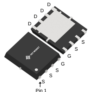
DFN5X6-8L
