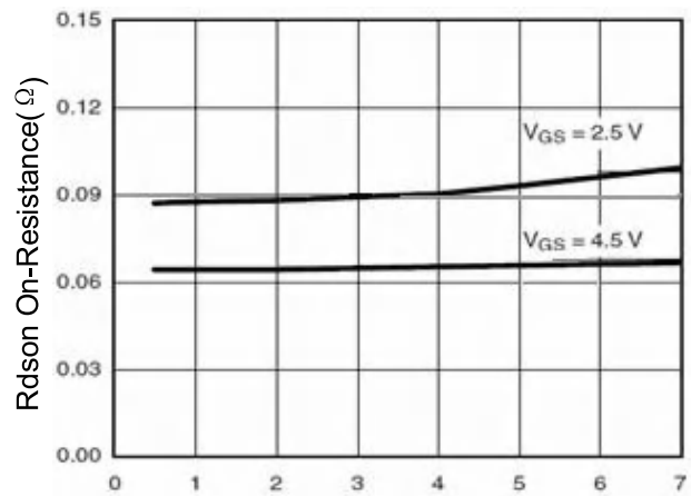
Figure 6 Drain-Source On-Resistance
