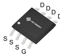
SOP-8 (SOIC-8)
