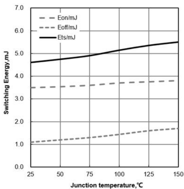
Figure 12. Typical Switching Energy vs Junction Temperature ( V_{CE}=600\text{V} , V_{GE}=15/0\text{V} , I_C=40\text{A} )
