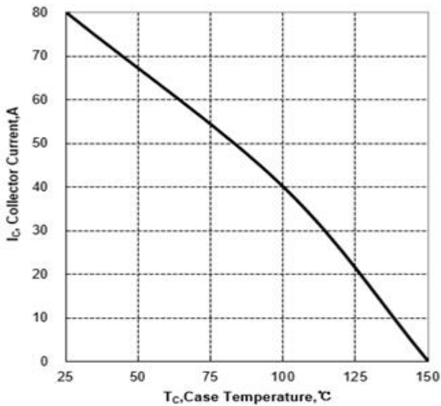
Figure 3. Collector Current vs Case Temperature
