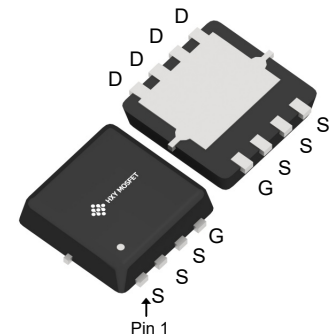
DFN3X3-8L (WDFN-8-EP(3.3x3.3))
