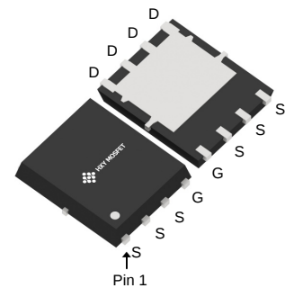
DFN5X6-8L (DFN-8(5x6))
