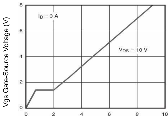
Figure 11 Gate Charge
