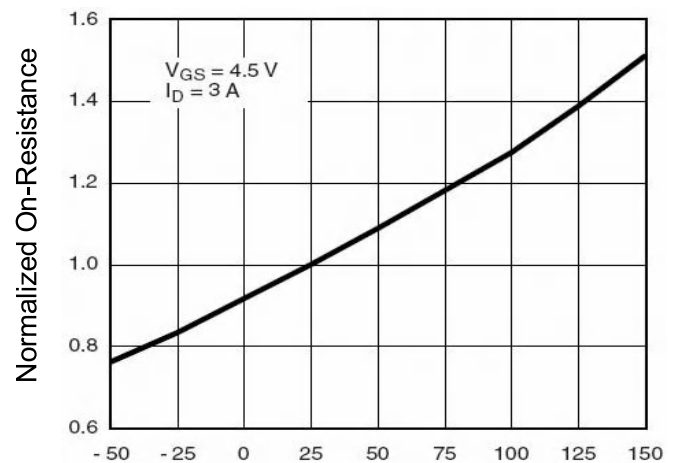
Figure 8 Drain-Source On-Resistance
