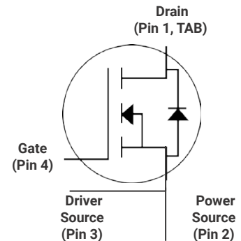
TO-247H-4L
