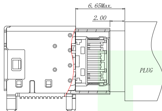
AFTER MATING
