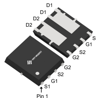
DFN5X6B-8L
