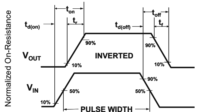
Figure 2: Switching Waveforms
