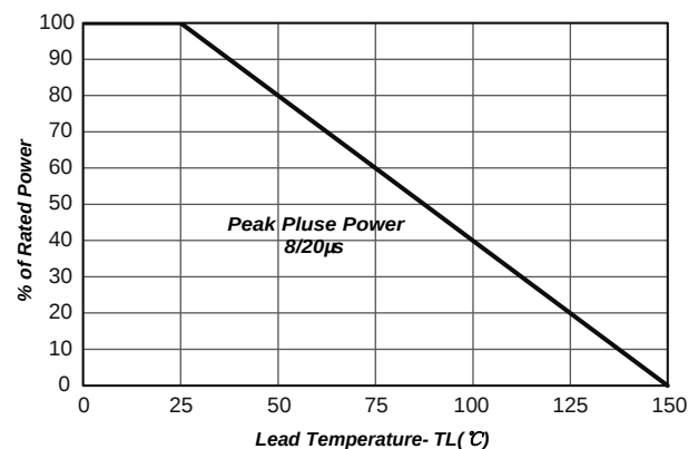
Fig3.Power Derating Curve
