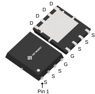
DFN5X6-8L (TDSO-8)
