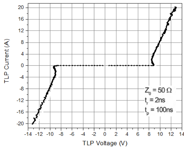
Fig1.TLP Measurement
