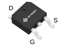
TO-252-2L (TO-252-2(DPAK))
