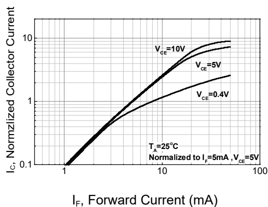
Figure 2: Normalized Collector Current vs Forward Current
